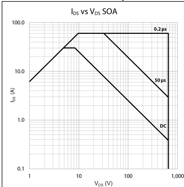
Figure 13: Safe Operating Area @ T_{case} = 25^\circ C
