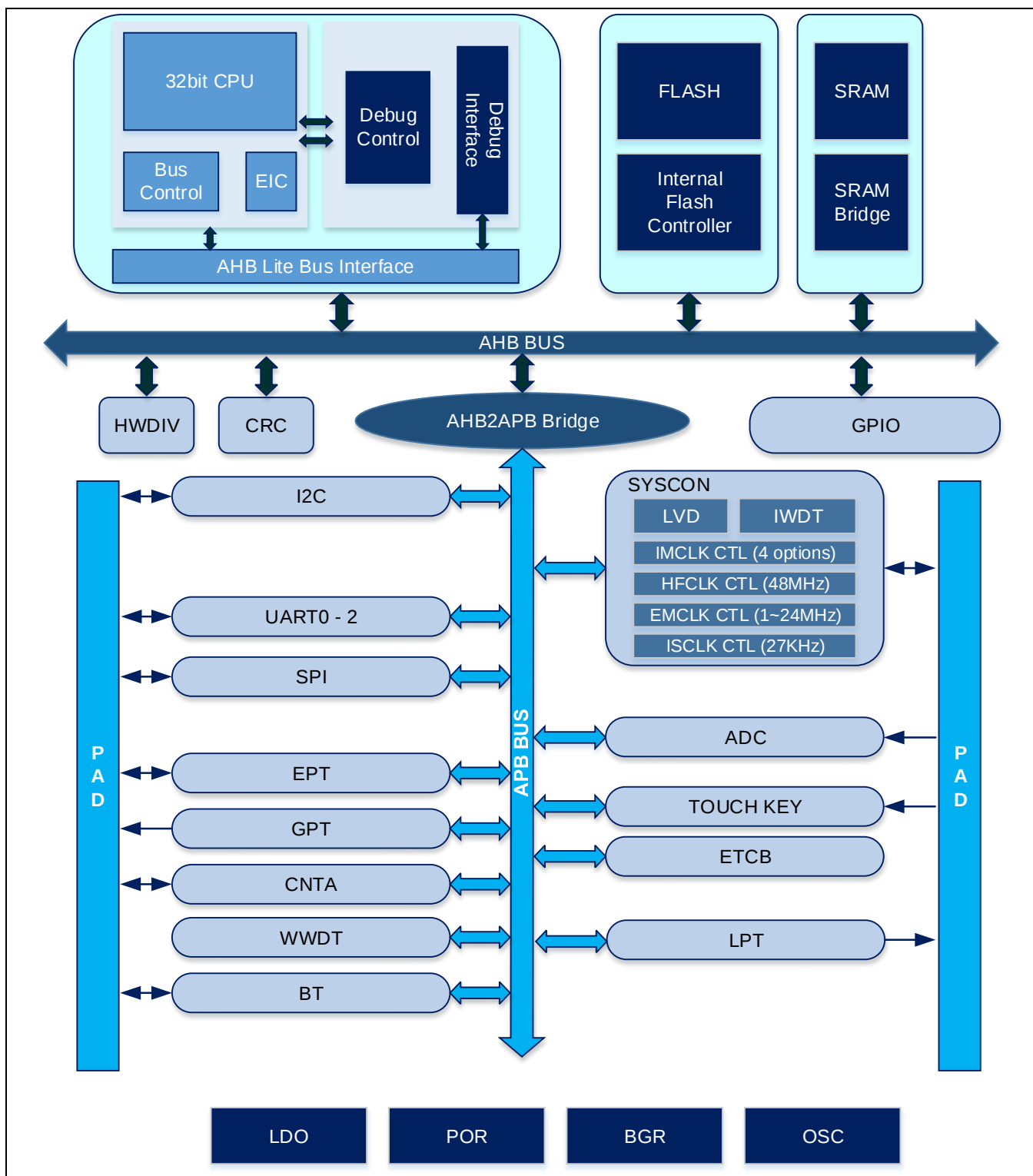
Figure 1-1 APT32S003F8PT模块框图
