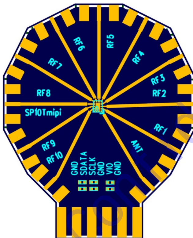
Figure 4 Evaluation Board Assembly Diagram
