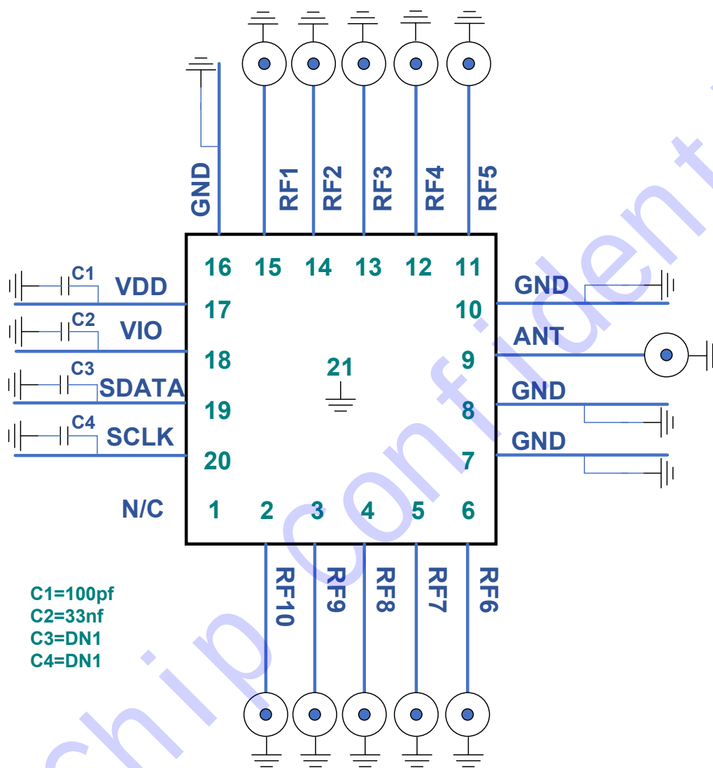
Figure 3 Application circuit
