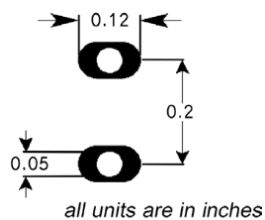
TO-220F-2L
