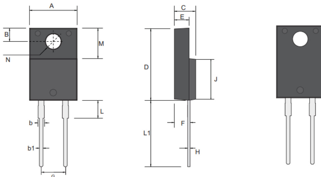
TO-220F-2L mechanical data
