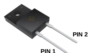
TO-220F-2L
