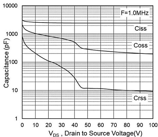
Fig.7 Capacitance
