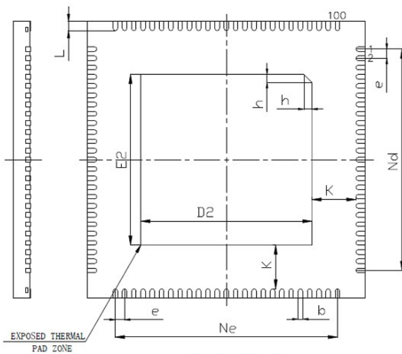
BOTTOM VIEW
