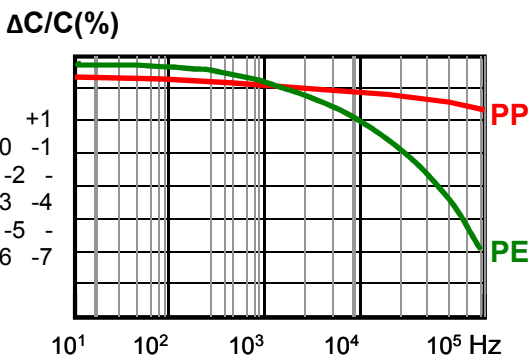
Frequency Characteristics
