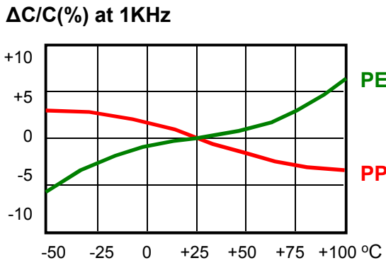
Temperature Characteristics
