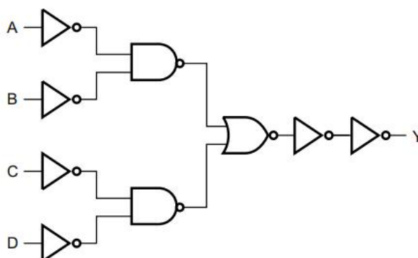
Figure 3.1: CD4002 Logic Diagram
