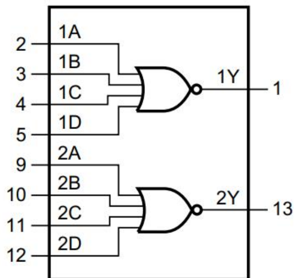
Figure 2.2 Functional Diagram
