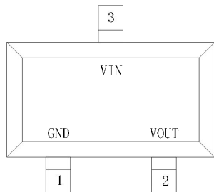
SOT23-3L (TOP VIEW)
