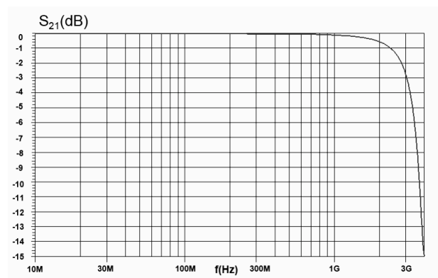
Figure 7. S 21 attenuation
