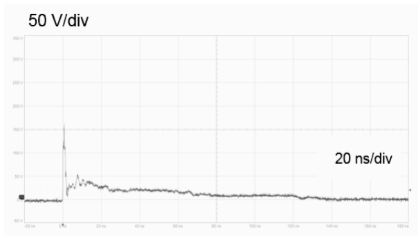
Figure 4. ESD response to ISO10605-C = 150 pF, R = 330 \Omega (+8 kV contact discharge) Figure 5. ESD response to ISO10605-C = 150 pF, R = 330 \Omega (-8 kV contact discharge)
