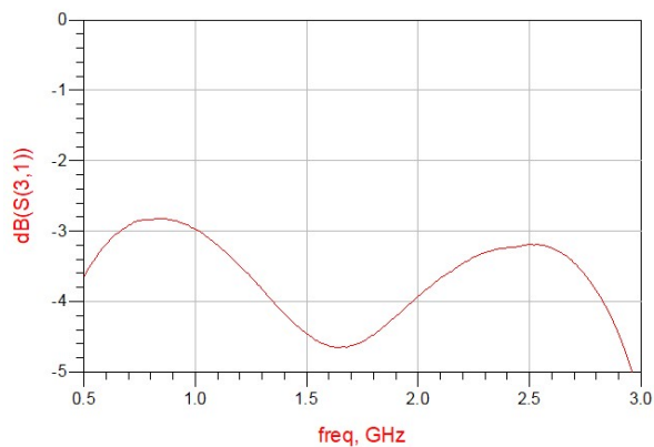
Figure 3. MHC0530W03 Coupling
