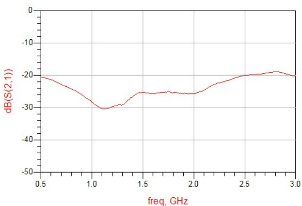
Figure 9. MHC0530W03 Isolation
