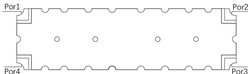
Figure 1. MHC0530W03 (Bottom View)
