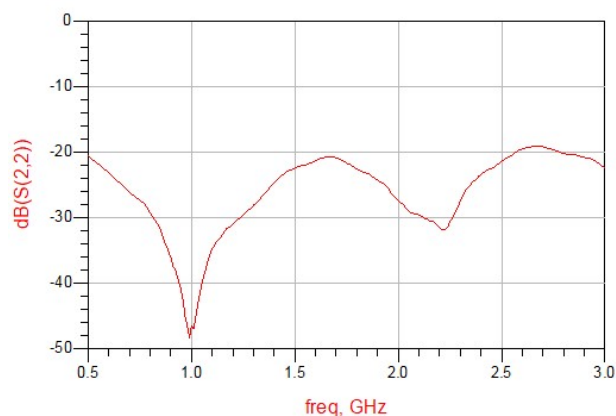
Figure 6. MHC0530W03 Return Loss (S22)
