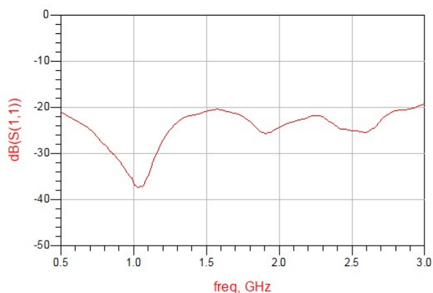
Figure 5. MHC0530W03 Return Loss (S11)
