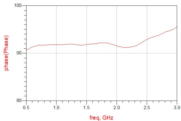
Figure 10. MHC0530W03 Phase
