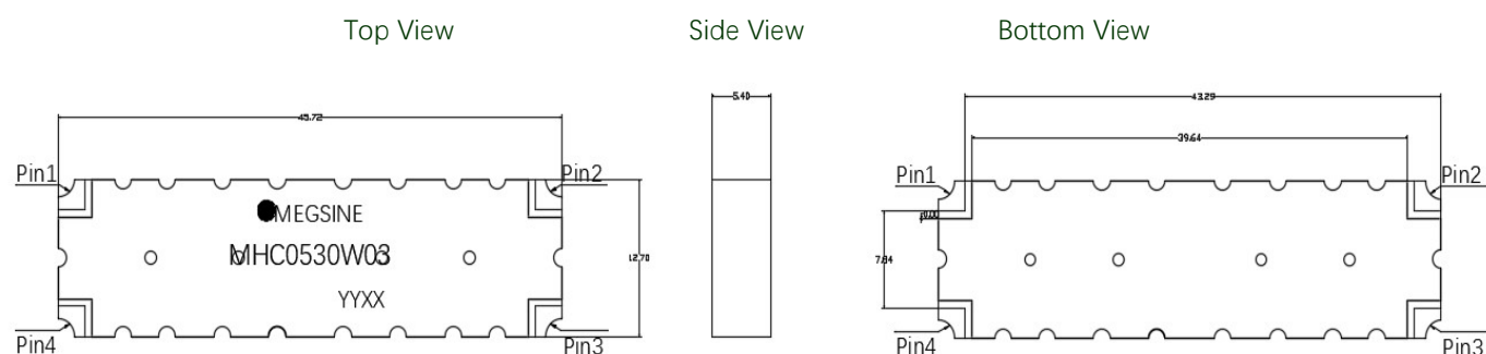
Figure 2. MHC0530W03 Outline Drawing
