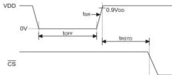
Figure 4 Power-on Reset Timing
