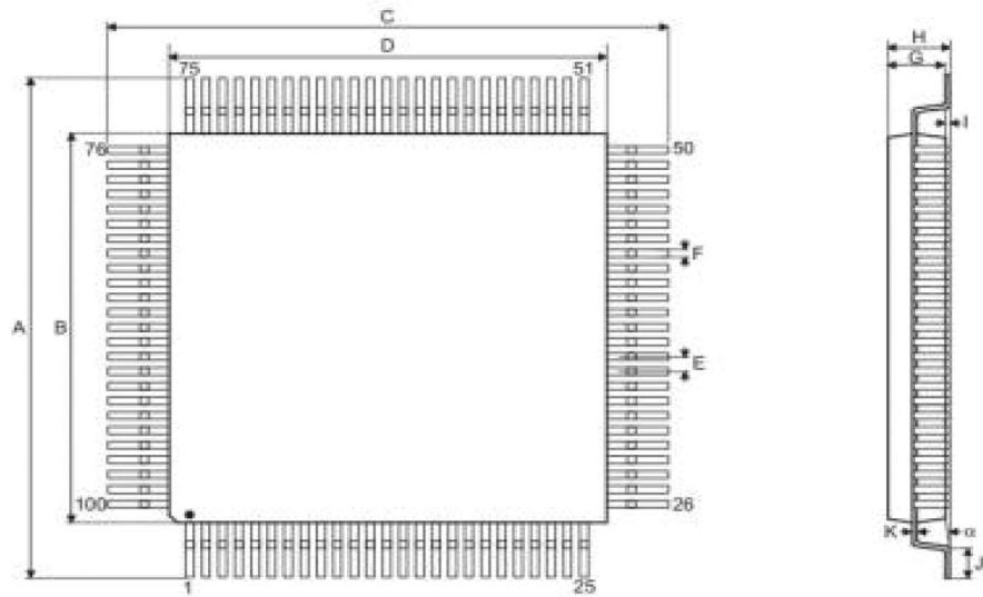
100-pin LQFP (14mm×14mm) Outline Dimensions
