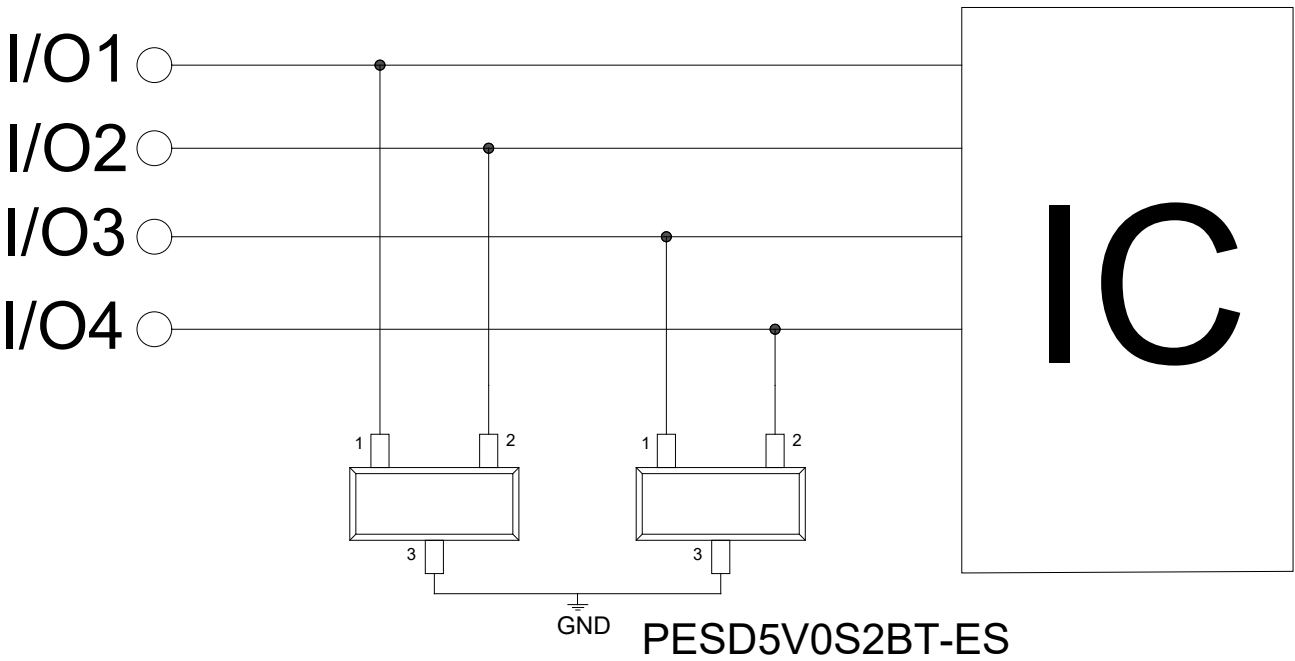
Typical Interface Application of CAN Bus Protection
