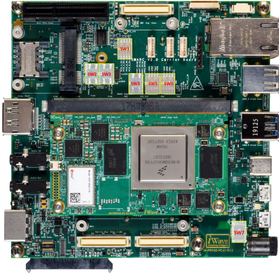
Figure 22: SMARC On Board Switches
