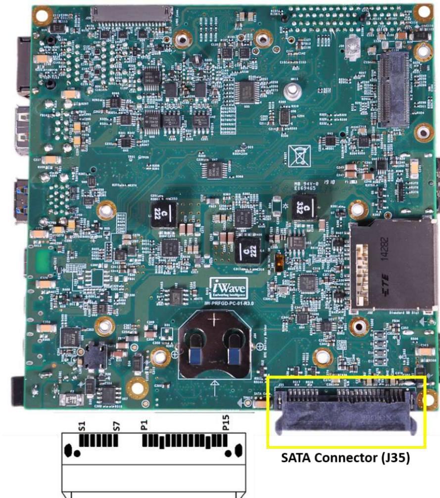
Figure 8: SATA Connector
