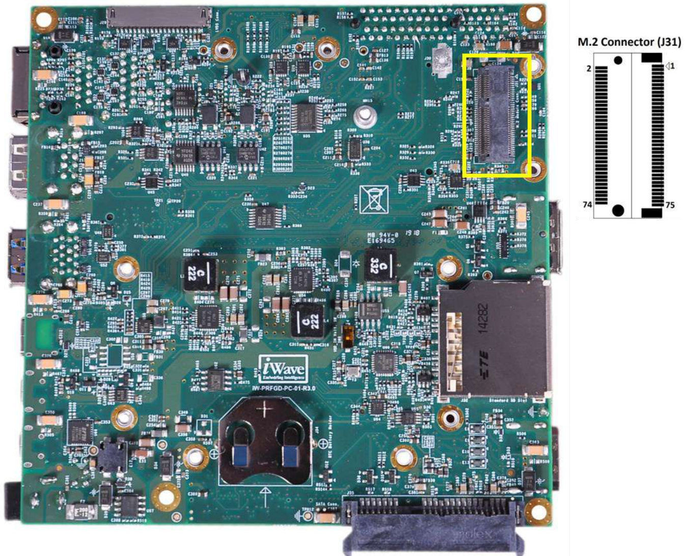
Figure 7: M.2 Connector
