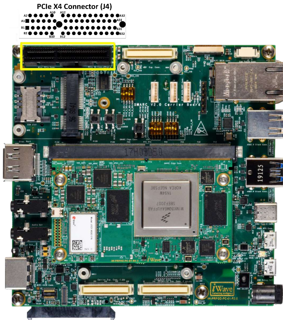
Figure 5: PClex4 Connector
