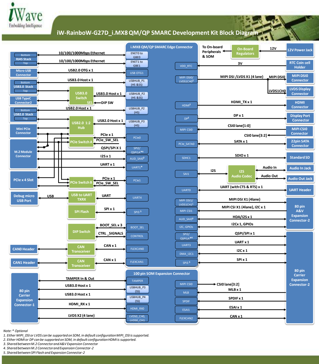
Figure 1: i.MX8 QM/QP SMARC Development Platform Block Diagram
