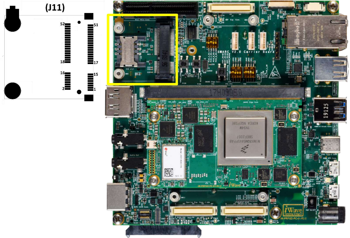
Figure 6: Mini PCIe Connector
