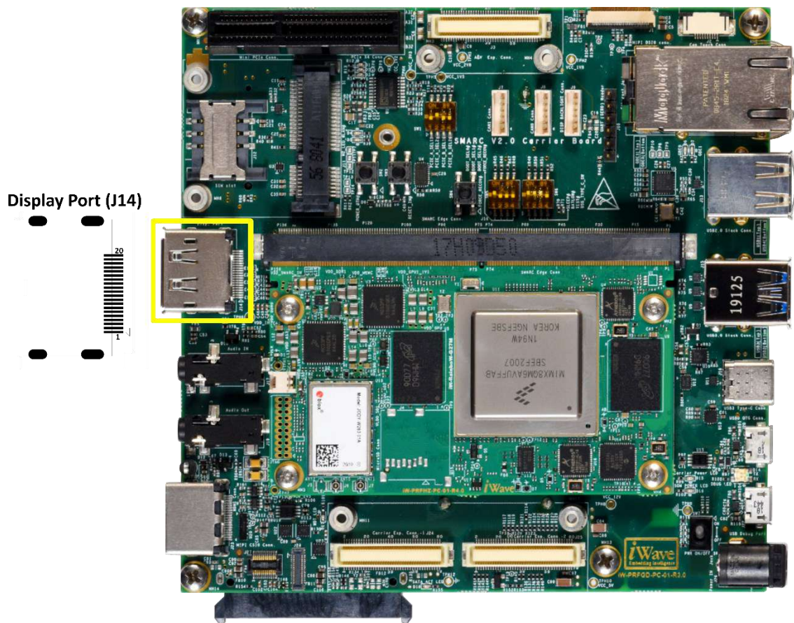
Figure 20: Display Port
