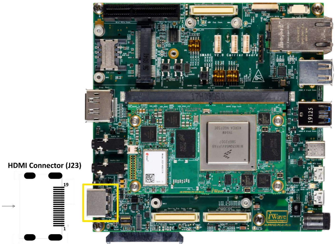
Figure 15: HDMI Output
