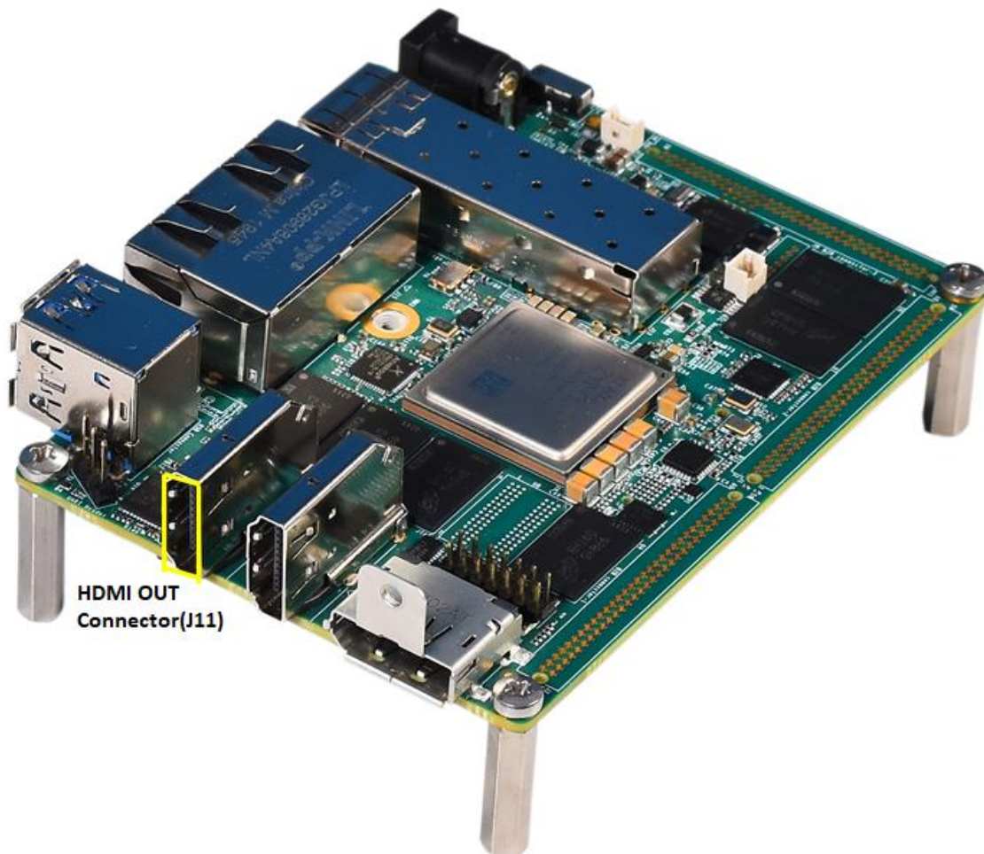
Figure 12: HDMI Out Connector
