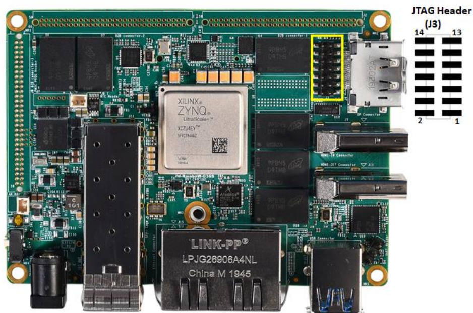
Figure 14: JTAG Header
