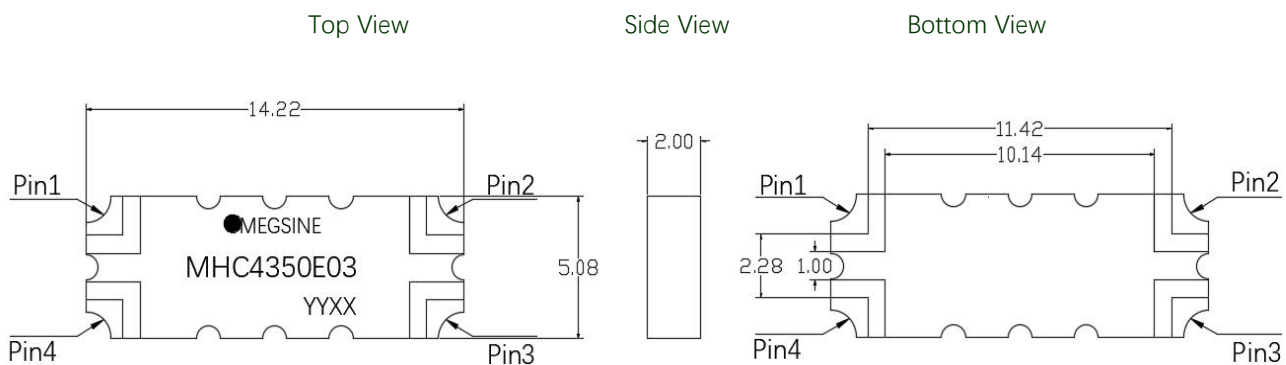
Figure 2. MHC4350E03 Outline Drawing
