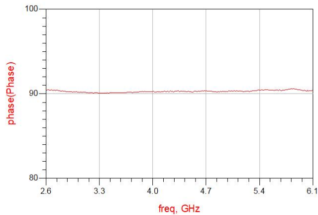
Figure 10. MHC4350E03 Phase
