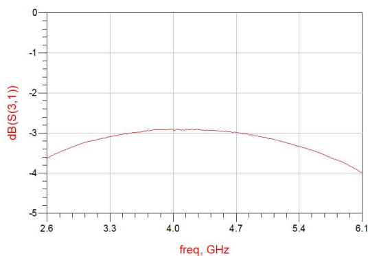
Figure 3. MHC4350E03 Coupling
