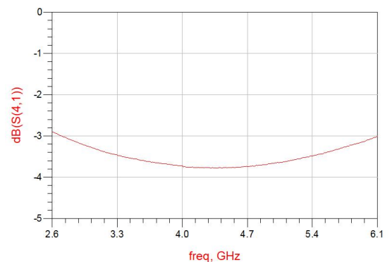
Figure 4. MHC4350E03 Transmission
