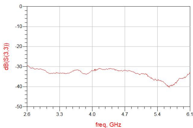
Figure 9. MHC4350E03 Isolation
