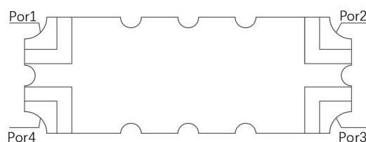
Figure 1. MHC4350E03 (Bottom View)
