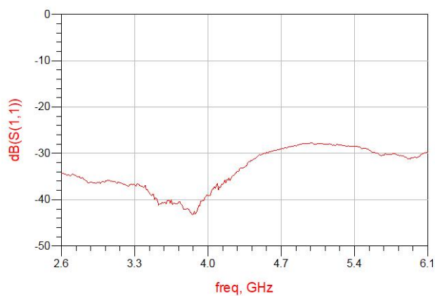
Figure 5. MHC4350E03 Return Loss (S11)
