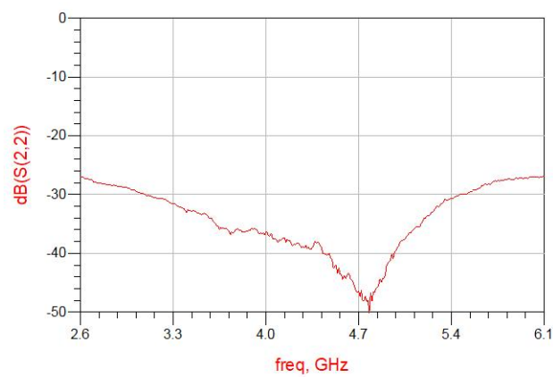
Figure 6. MHC4350E03 Return Loss (S22)
