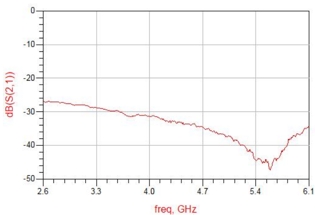
Figure 9. MHC4350E03 Isolation
