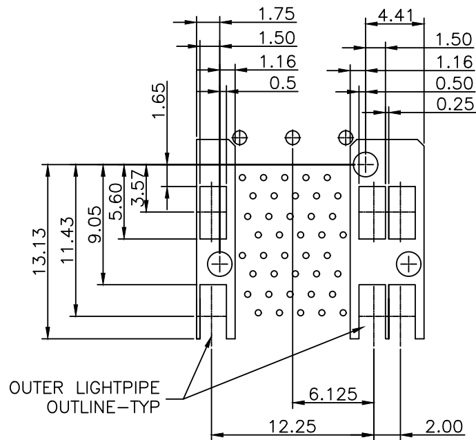
DETAIL-KEEPOUT ZONES
