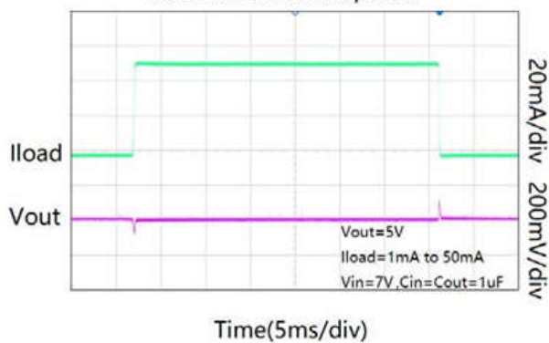
Load-Transient Response
