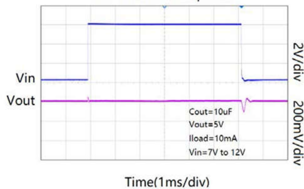
Line-Transient Response
