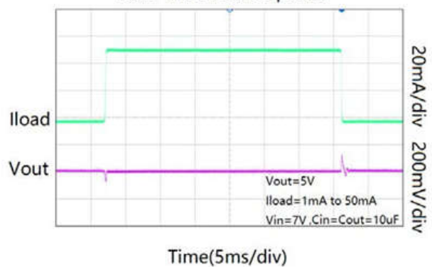
Load-Transient Response
