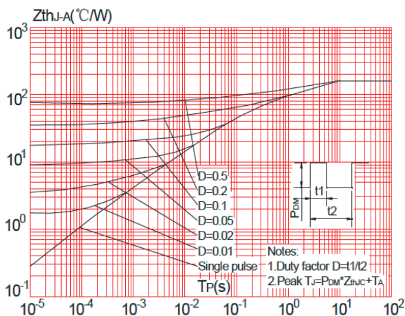
Figure 7: Maximum Effective Transient Thermal Impedance vs. Pulse Width
