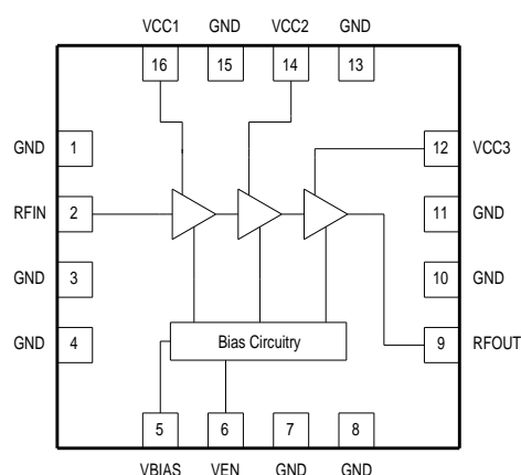
Figure 2. GDM4028 Function Block Diagram
