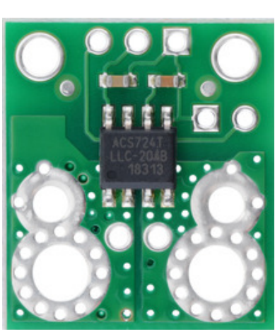
ACS724LLCTR-20AB Current Sensor Carrier -20A to +20A, top view.
