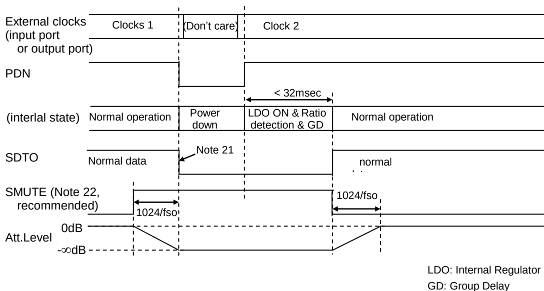
Figure 41. Sequence of Changing Clocks (Parallel Control Mode, PSN pin="H")
