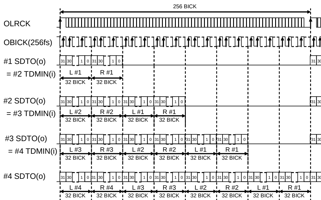
Figure 36. TDM Cascade
