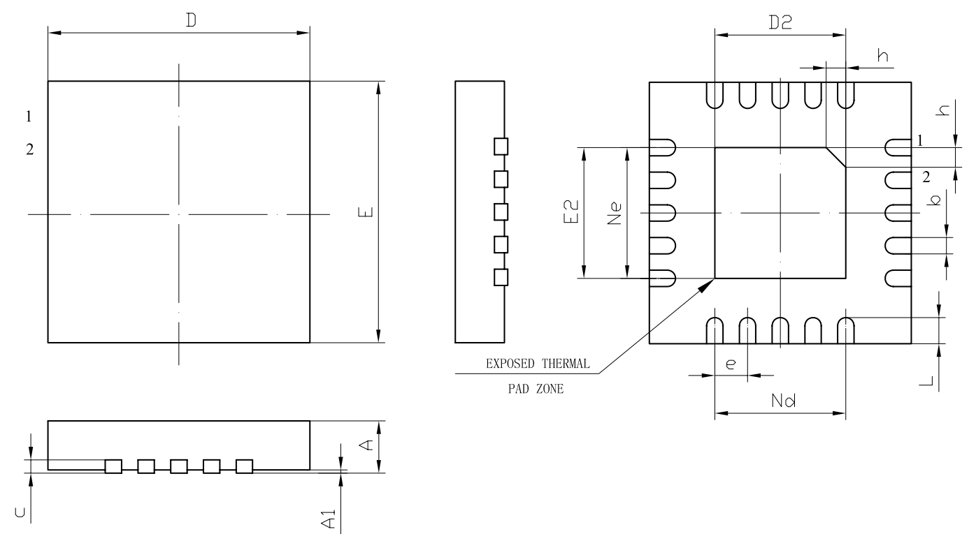
QFN20
