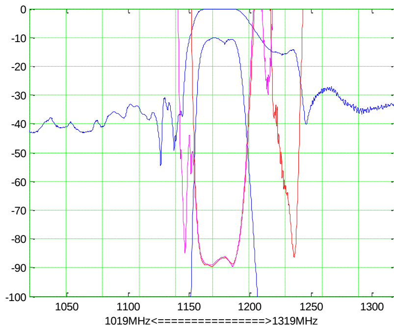
Frequency Response
