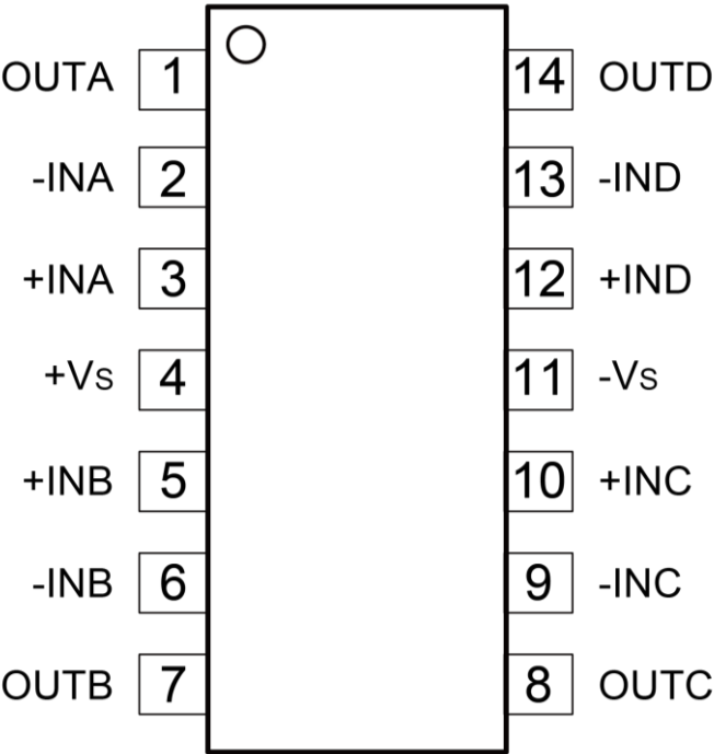
Figure 3. ZJA3000-4 Pin Configuration (14-lead SOIC and TSSOP)
