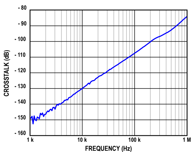
Figure 25. Channel Separation vs. Frequency
