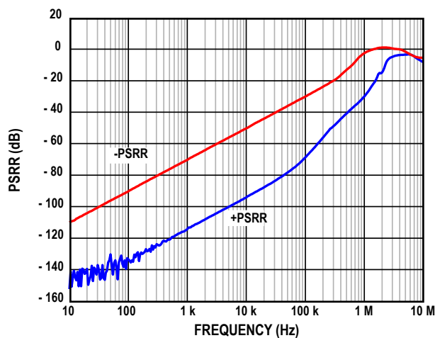
Figure 23. Power Supply Rejection Ratio (PSRR) vs. Frequency
