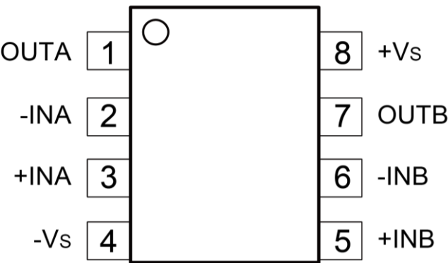
Figure 2. ZJA3000-2 Pin Configuration (8-lead SOIC and MSOP)
