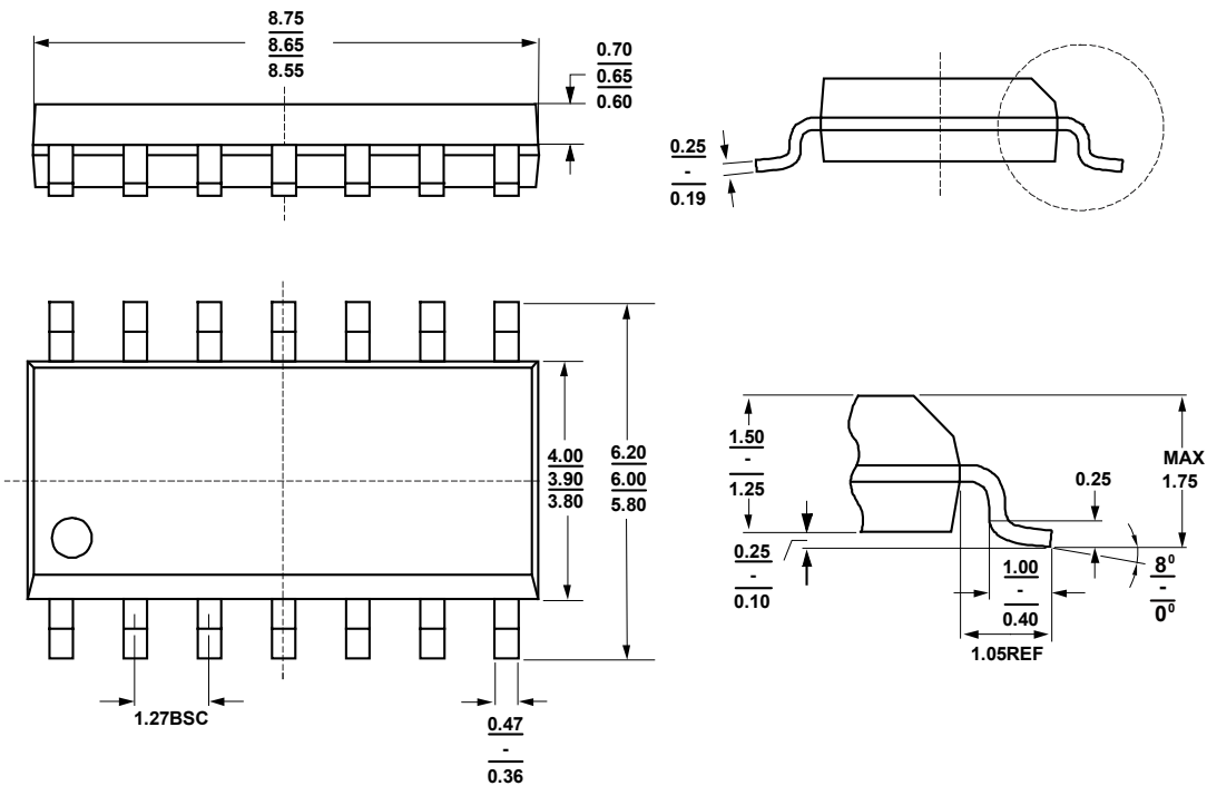
Figure 48. 14-Lead SOIC Package Dimensions shown in millimeters
