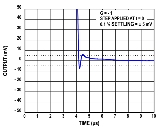
Figure 27. Negative Settling Time to 0.1%
