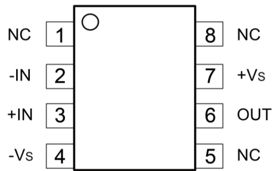
Figure 1. ZJA3000-1 Pin Configuration (8-lead SOIC and MSOP)
