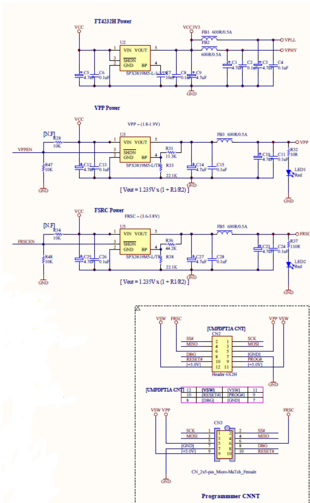
Figure 6.2 - Schematic part 1
