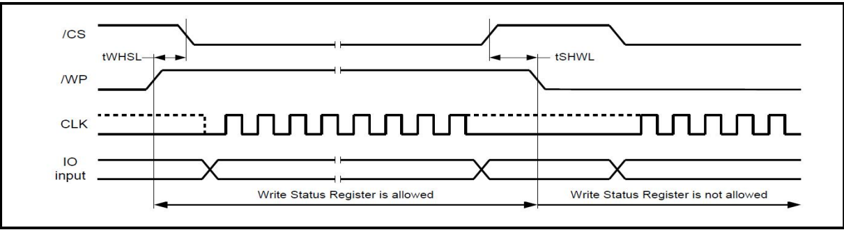
Figure 77. /WP Timing
