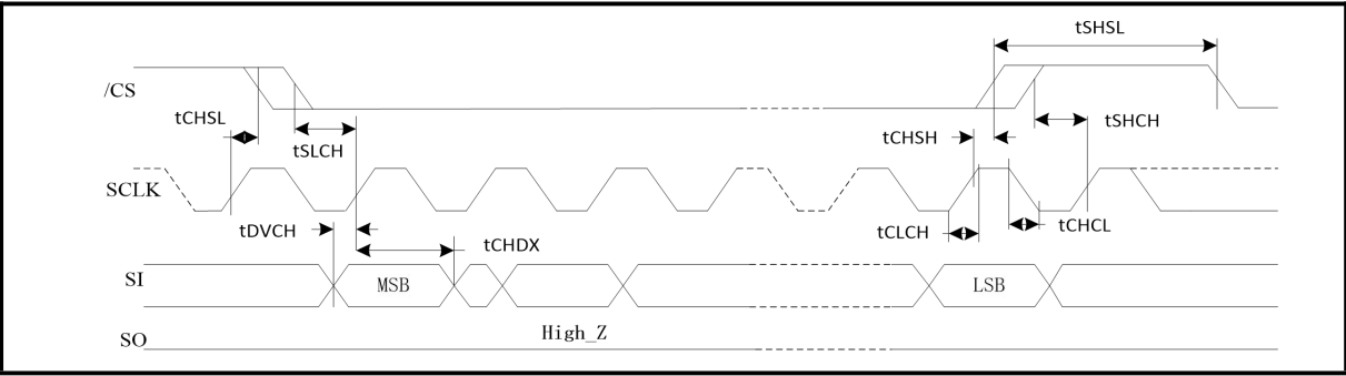
Figure 75. Output Timing
