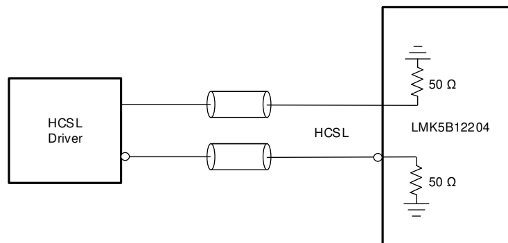
图 9-12. DC-Coupled CML (Source Terminated) to Reference (PRIREF/SECREF) or XO Inputs
