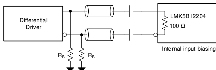
图 9-14. AC-Coupled Differential to Reference (PRIREF/SECREF) or XO Inputs
