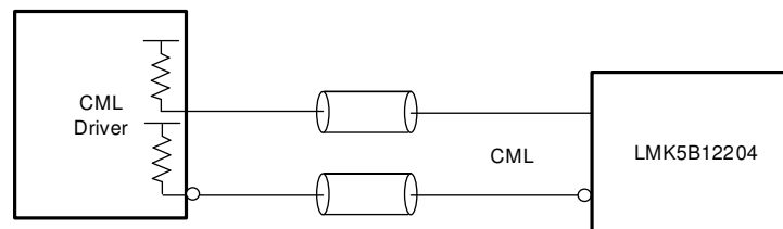
图 9-11. DC-Coupled LVDS to Reference (PRIREF/SECREF) or XO Inputs
