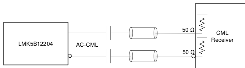
图 9-28. AC-CML Output to CML Receiver With Internal Termination/Biasing
