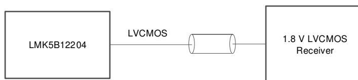
图 9-26. 1.8-V LVCMOS Output to 1.8-V LVCMOS Receiver
