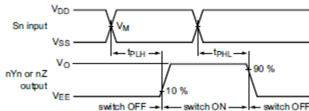
Figure 8. S_n to nYn, nZ propagation delays
