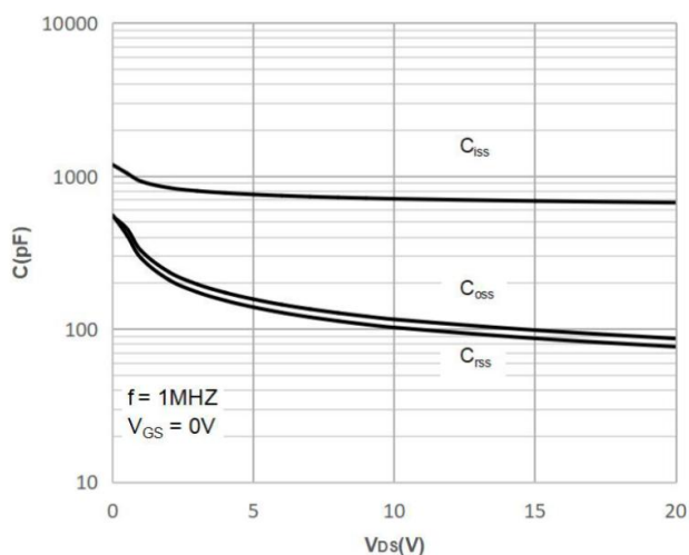
Figure 5: Capacitance Characteristics
