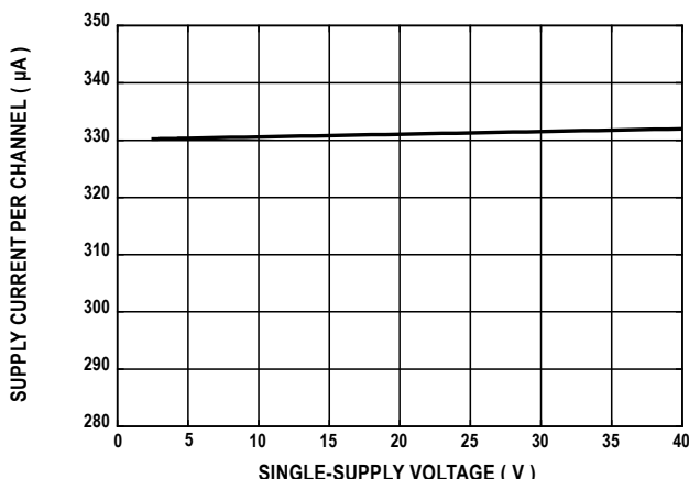
图26. 电源电流与单电源电压的关系( V_{IN} = 0\text{ V} , V_{REF} = 0\text{ V} )
