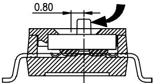
[推钮行程]
