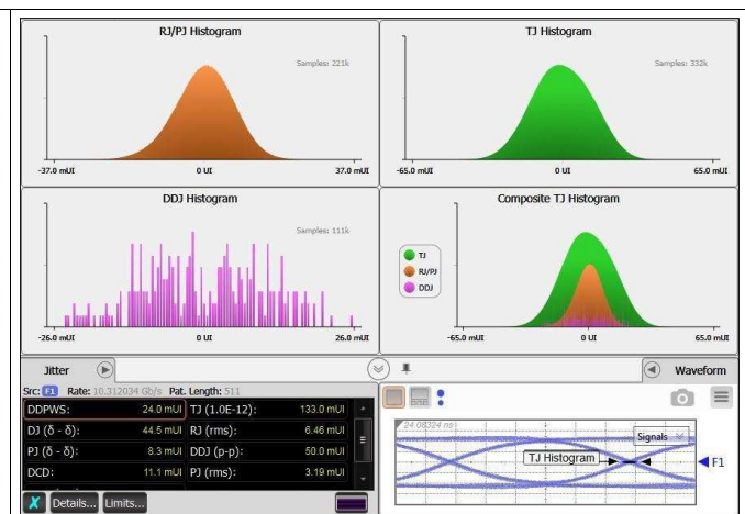
Figure 36. nPPI Jitter Performance with 5 Inch 4-Mil FR4 Input Trace, Test Pattern = PRBS-9, 10.3125 Gbps
