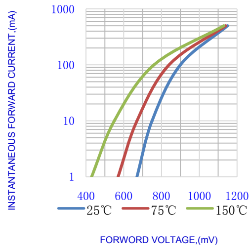
Fig.2- Forward characteristics
