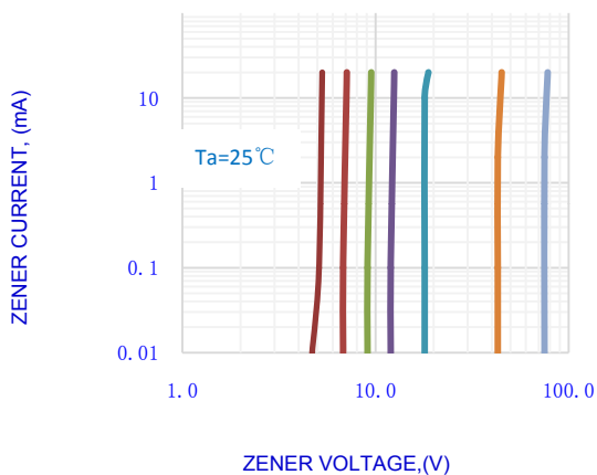
Fig.5-ZENER BREAKDOWN CHARACTERISTICS
