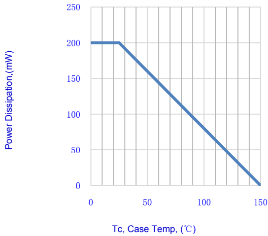
Fig.1-POWER DISSIPATION VS. AMBIENT TEMP.
