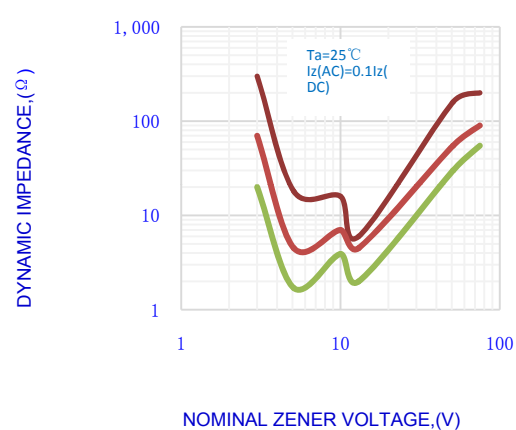
Fig.6-EFFECT OF ZENER VOLTAGE ON ZENER IMPEDANCE
