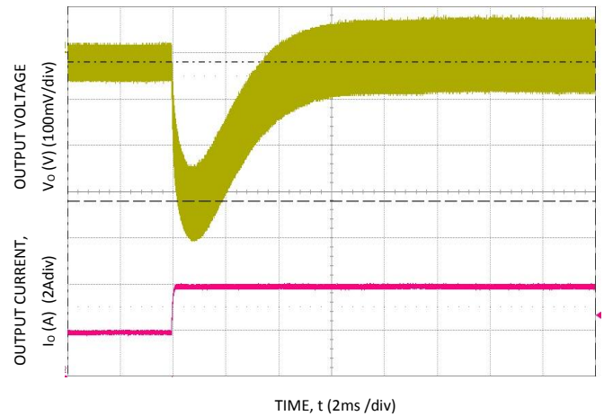
Figure 4. Transient Response to Dynamic Load Change from 50% to 100% at 12Vin, C_{out}=3 \times 10 \mu F + 470 \mu F , C_{Tune}=1000pF , R_{Tune}=30.1k\Omega
