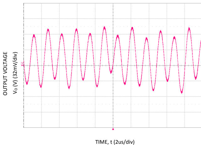
Figure 15. Typical output ripple and noise ( C_o=3 \times 10 \mu F + 470 \mu F , V_{IN} = 12V , I_o = I_{o,max} ).
