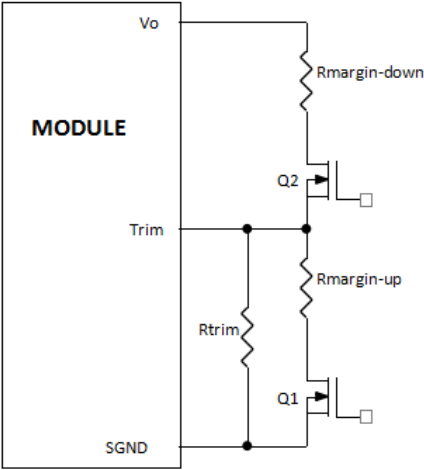
Figure 29. Circuit Configuration for margining Output voltage.
