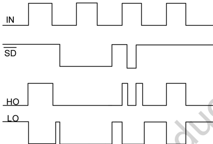
Figure 6-1 IR2104S Input and output timing waveform
