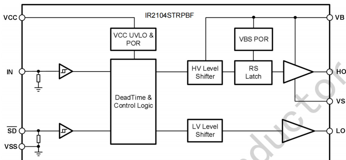
Figure 7-1 Function Block Diagram of IR2104S
