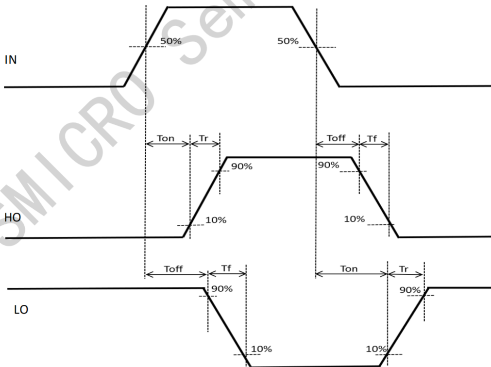
Figure 6-2 Propagation Time Waveform Definition
