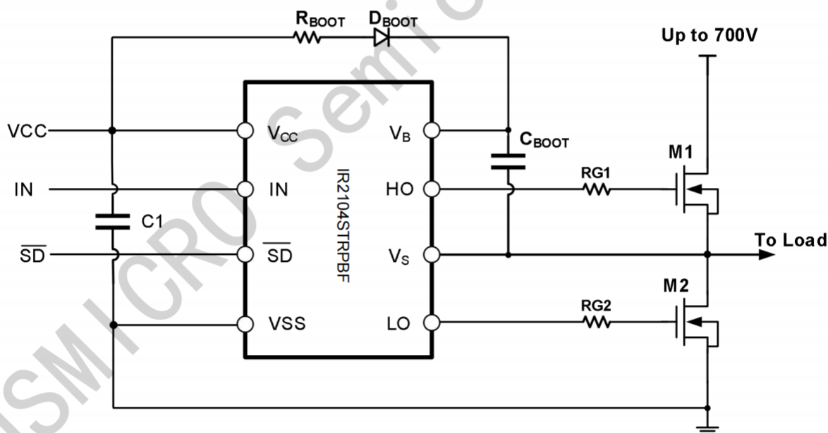
Figure 7-2 Typical application circuit of IR2104S
