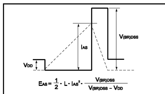
Fig.12 Avalanche Waveform
