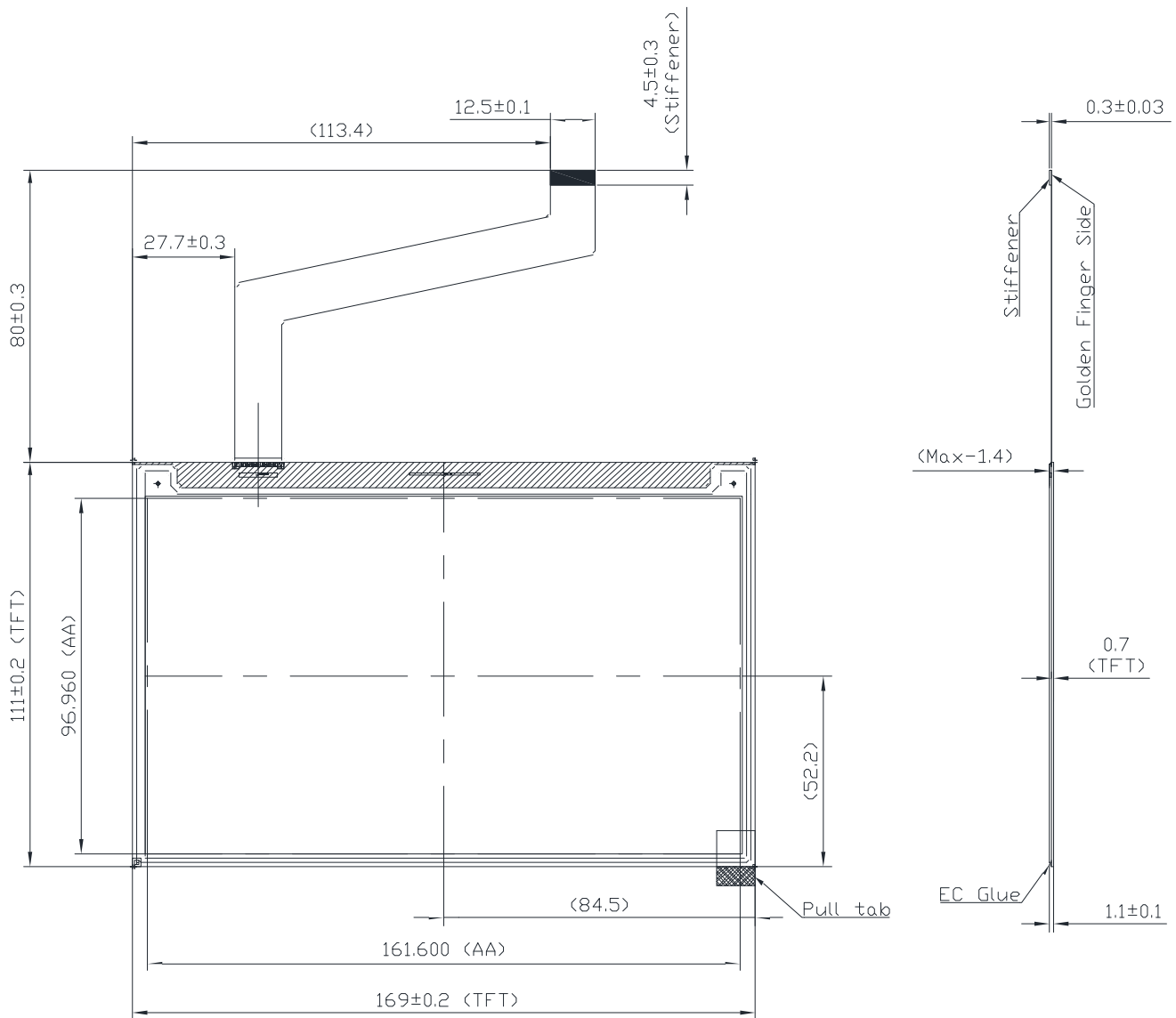
Figure 1-1 EPD Drawing
