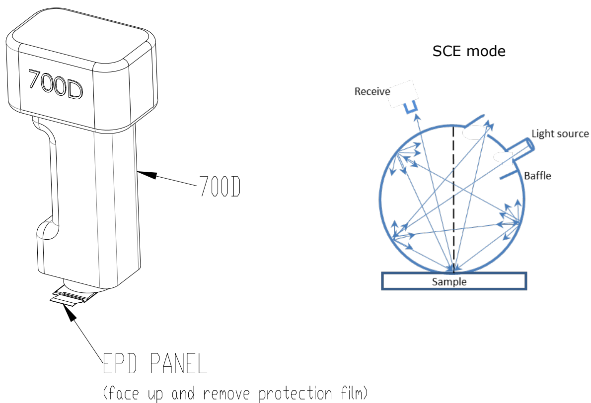
Figure 6-1 Optical Measurement
