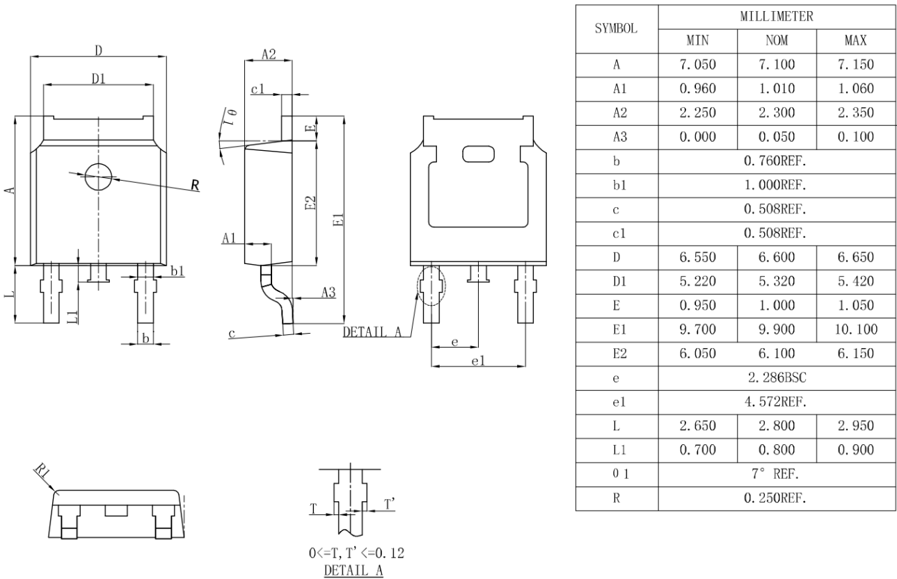
Figure 4. TO-252
