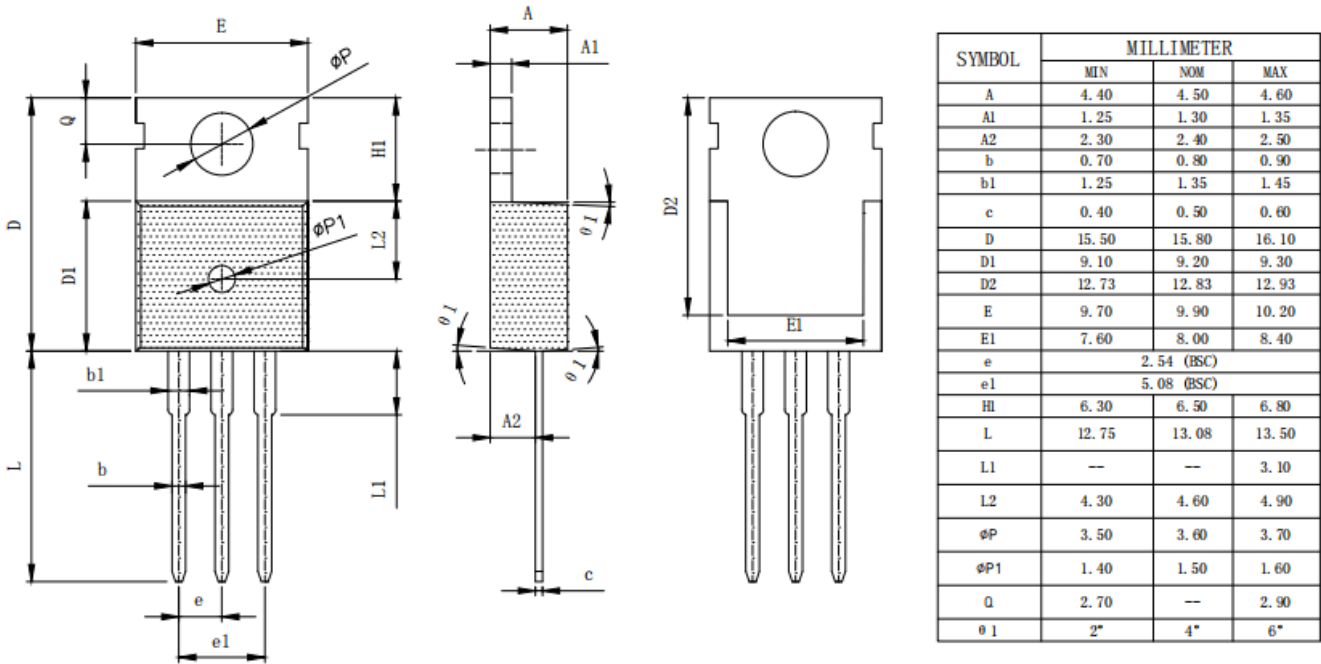
Figure 5. TO-220-FB
