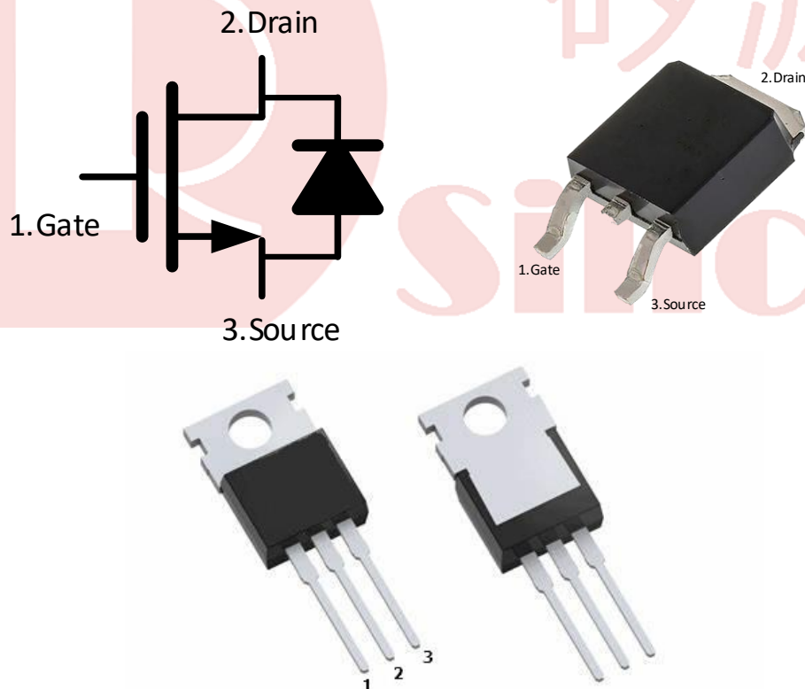
Figure 1. View and Internal Schematic Diagram
