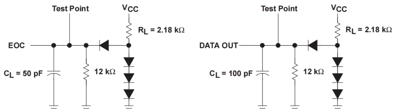
Figure 2. Load Circuits
