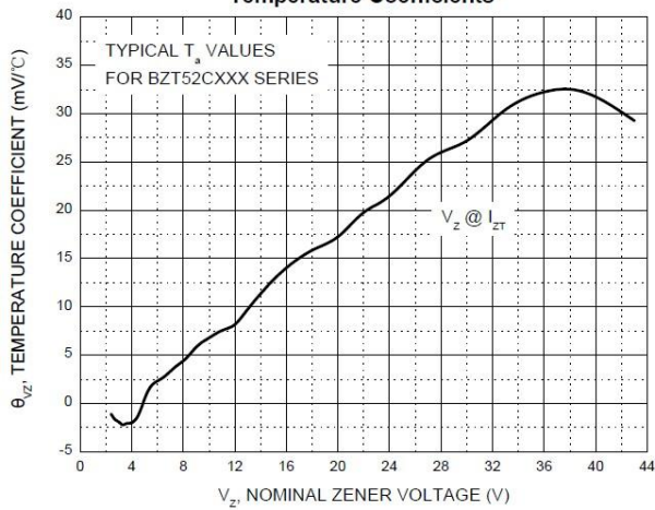
Temperature Coefficients
