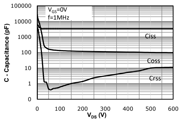
Fig 11: Capacitance Characteristics
