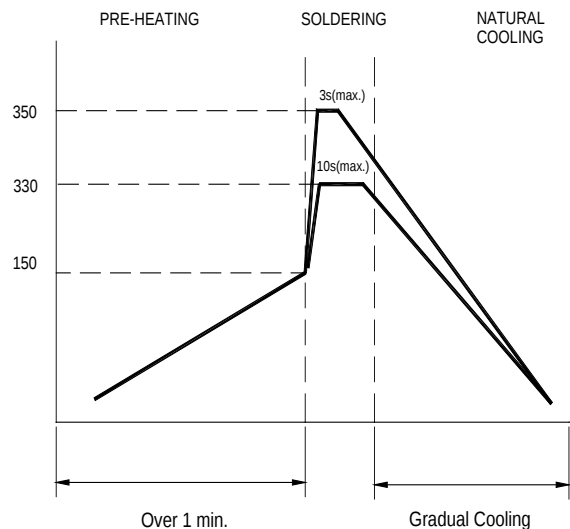
Figure 2. Hand Soldering
