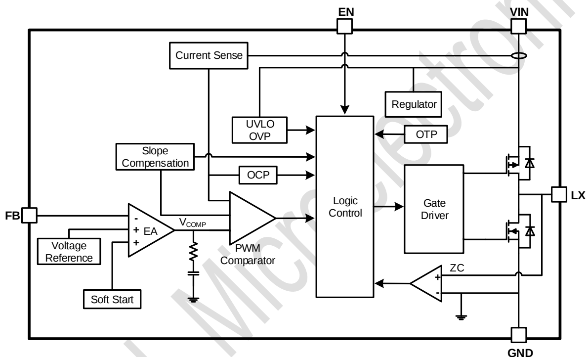
Figure 2. TMI3108 Block Diagram
