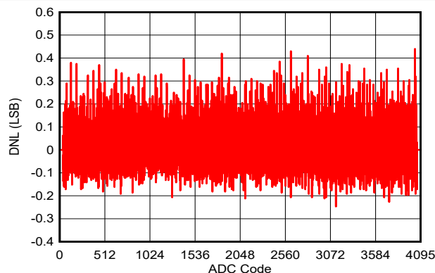
图 7-32. DNL vs. ADC Code ( V_{in} = 3V Sine Wave, Internal Reference, 200ksps)
