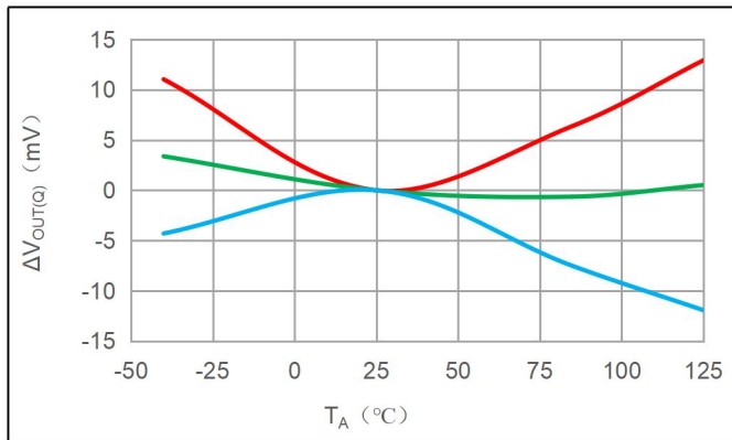
\Delta V_{OUT(Q)} vs. T_A
