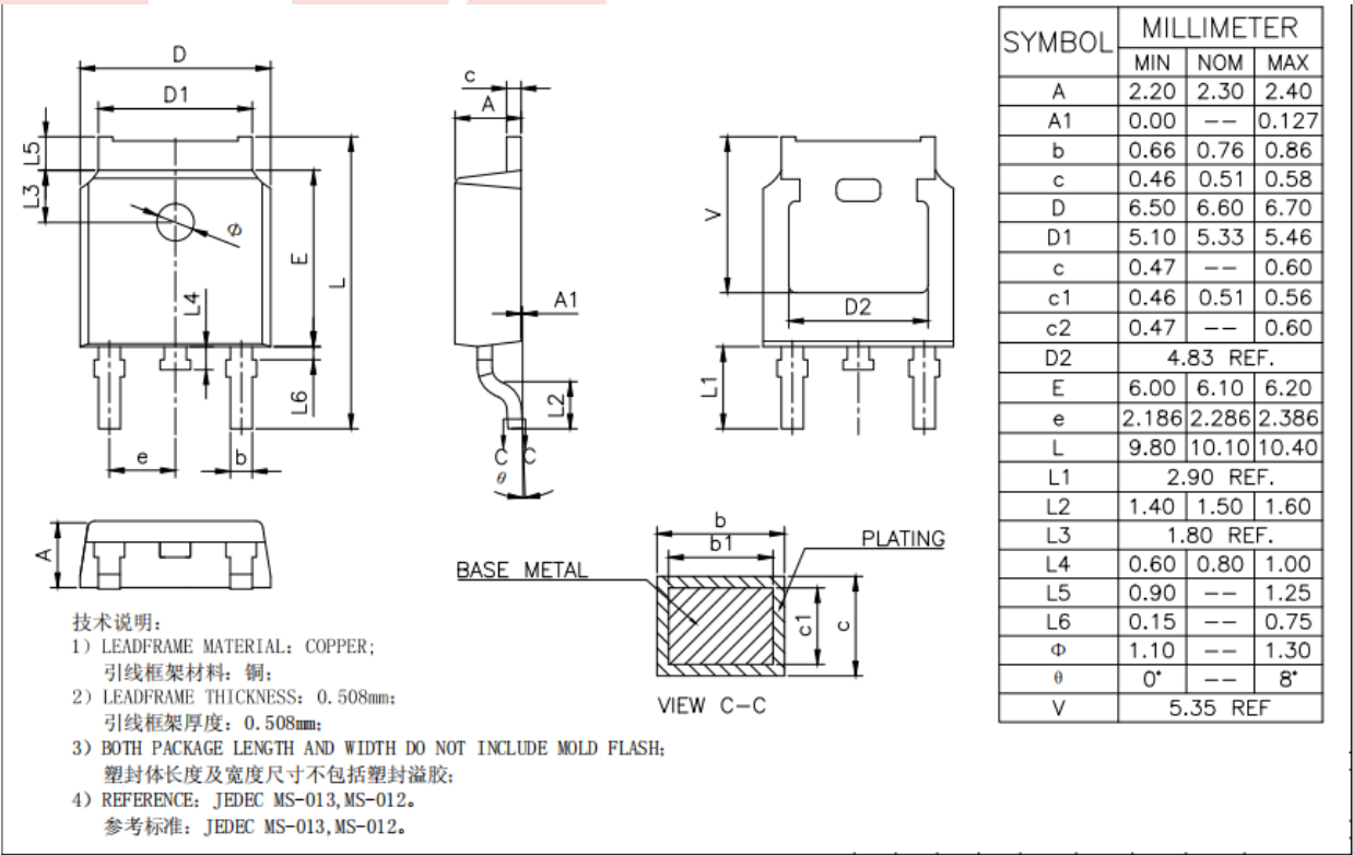
Figure 4. TO-26
