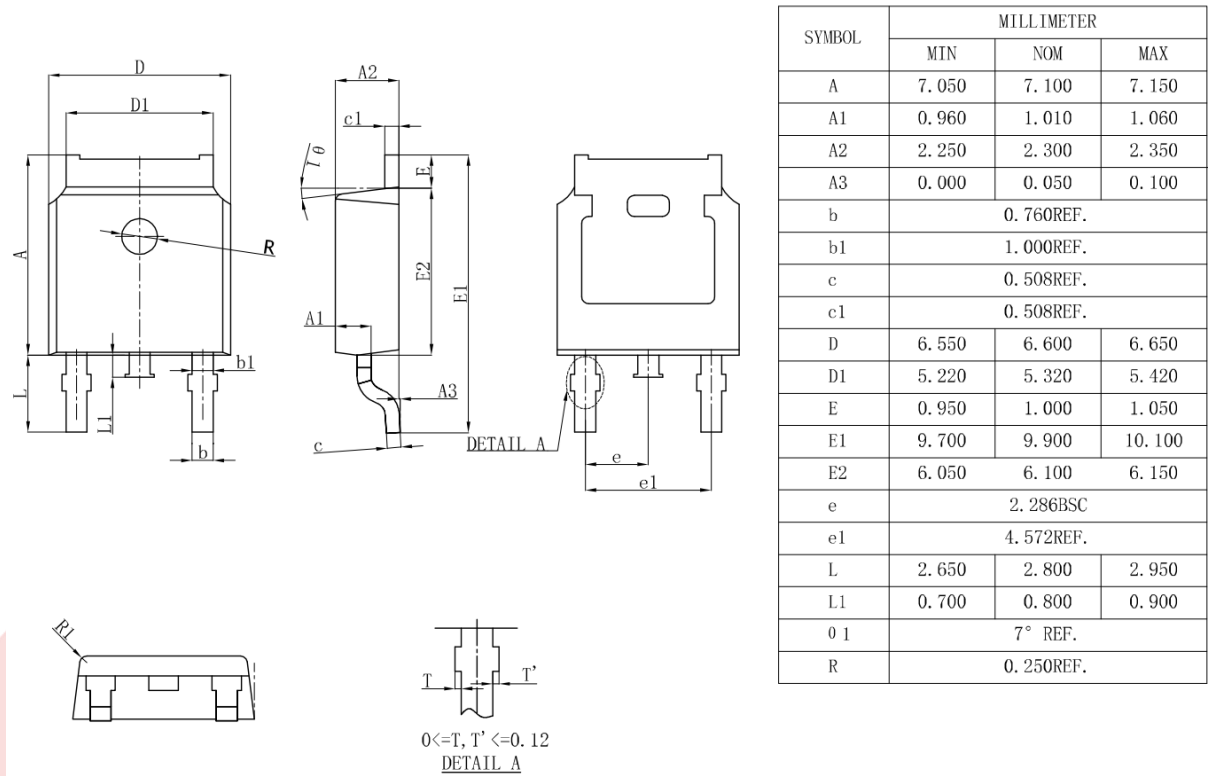
Figure 4. TO-252
