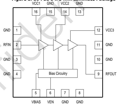
Figure 2. GDM2628 Function Block Diagram
