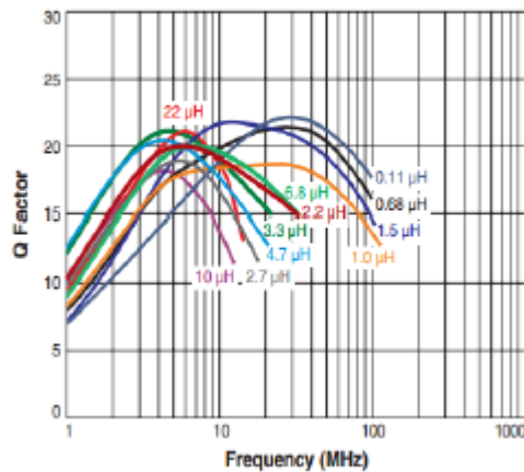
Typical Q vs Frequency
