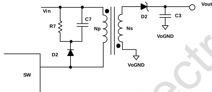
Figure 8 RCD snubber
